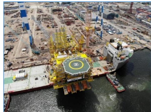
BOKOR CPP Phase 3 Redevelopment Project - Loadout and Sail away (Aug 2020)
